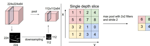
Figure 2. pooling layer
