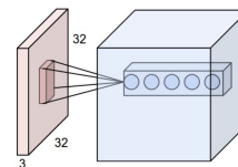
Figure 1. conv layer
